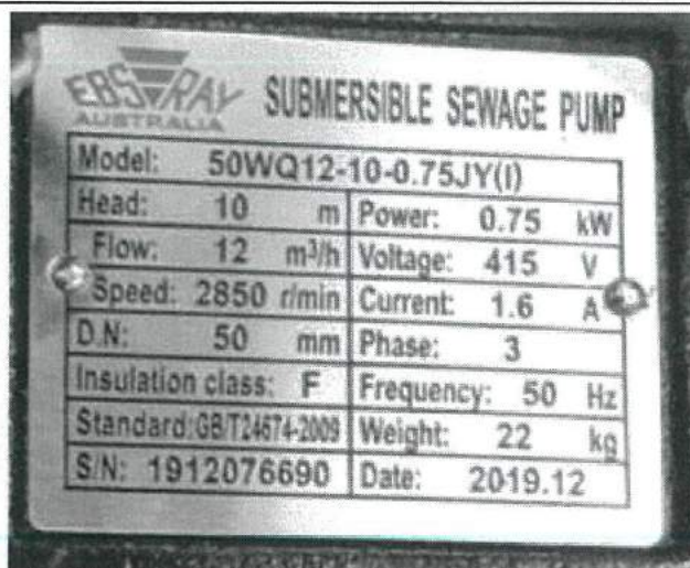
Figure 5: Name plate on pump tested.
